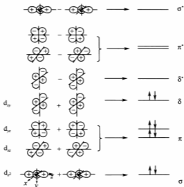
图6 Re-Re键中电子组态
