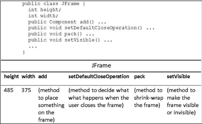
Figure 20-2: A simplified depiction of the JFrame class.
