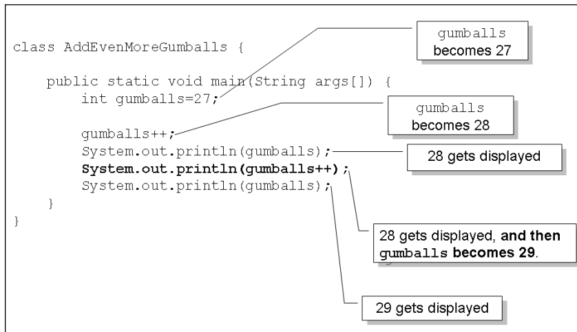
Figure 7-11: Using postincrement.
