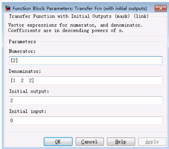
图 6-13 Transfer Fcn (with initial outputs) 模块设置
